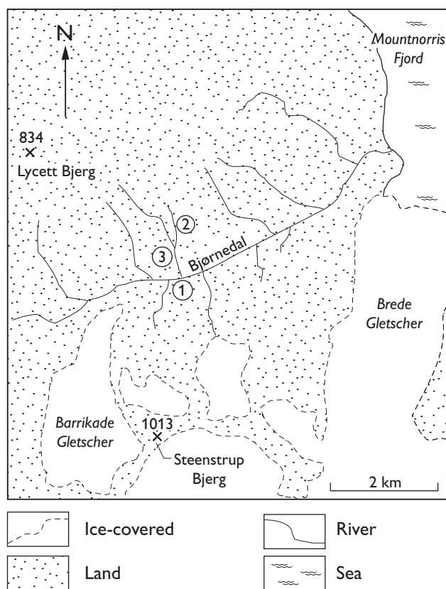
Fig. 2. Map of the Bjørnedal area, Trail Ø showing locations of sections and ammonite localities. 1 , Locality 1 with section JTH-15/96; 2 , Locality 2 with section JTH-14/96; 3 , Locality 3. Altitude of mountains in metres.
